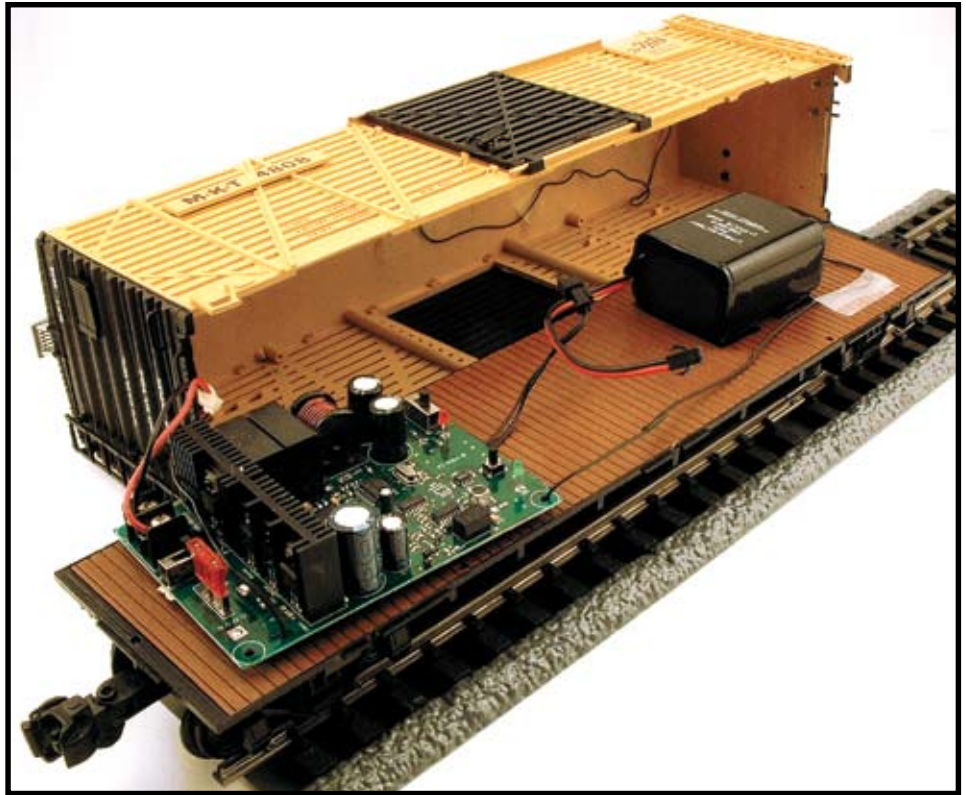
CRE-55496 Trailing RC Car with Train Engineer receiver installed
