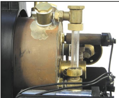
Water Sight Glass
