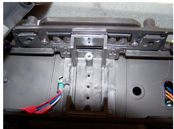
The pedestal with the nut attached. These will add about 3/16 th of an inch in height.
